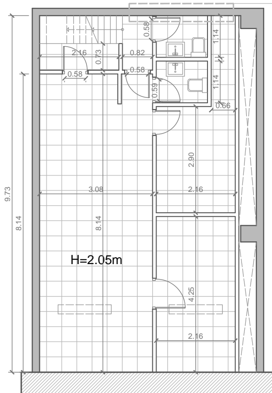
SOTOKO SOLAIRUA A_{\text{erabilgarria}} = 49.30 \text{ m}^2 A_{\text{eraikia}} = 62.45 \text{ m}^2
