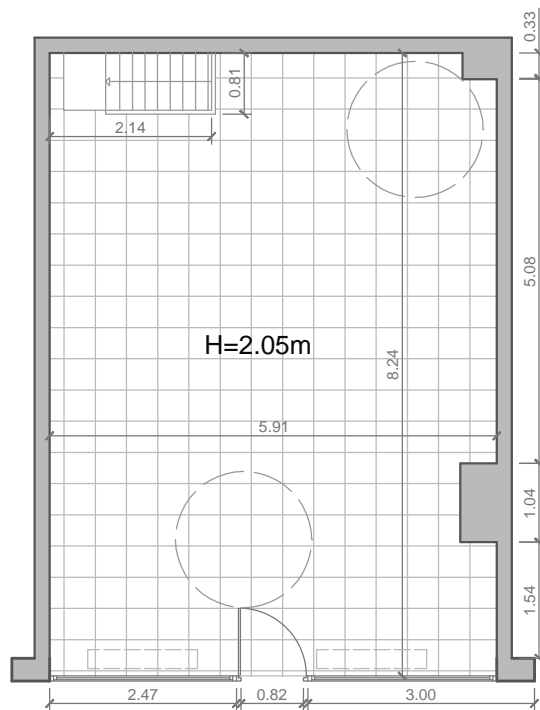
SOTOKO SOLAIRUA A_{\text{erabilgarria}} = 49.30 \text{ m}^2 A_{\text{eraikia}} = 62.45 \text{ m}^2
